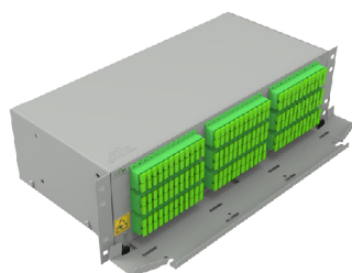
PS-19/HD 3U Fibre Optic Patch Panel
