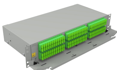
PS-19/HD 2U Fibre Optic Patch Panel
