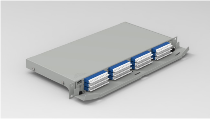
PS-19/144LC/1U Fibre Optic Patch Panel
