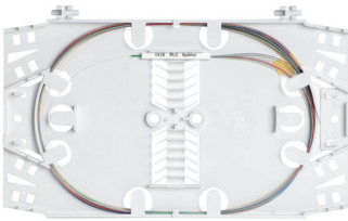
KS-24 splice tray with built in PLC 1x16 splitter
