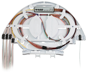
KSH splice tray with built in PLC 1x16 splitter
