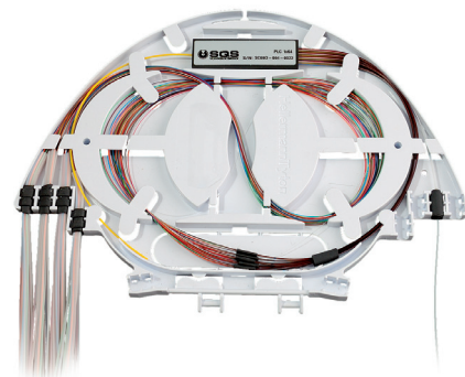
KSH splice tray with built in PLC 1x16 splitter
