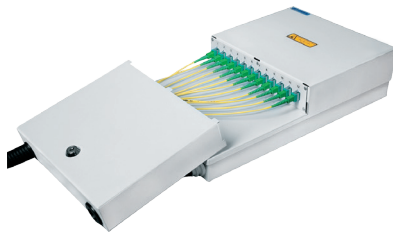
Fibre optic distribution box PS-5/24/P with adapter plate lid
