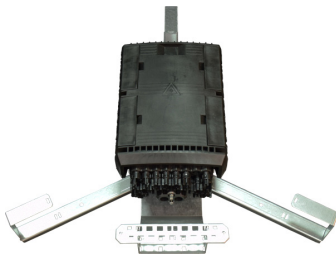
Aerial closure OSS-ZSD-48/24
