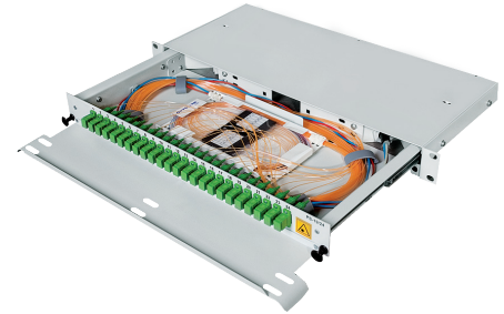
19" Patch Panel PS-19 with PO-2
